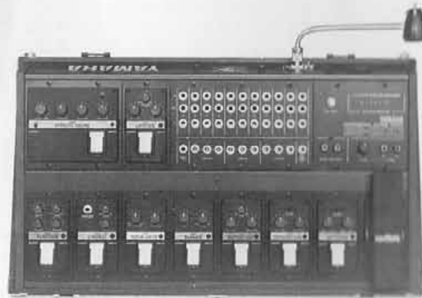
PROFESSIONAL SYSTEM BOARD SB-200 ㉘
